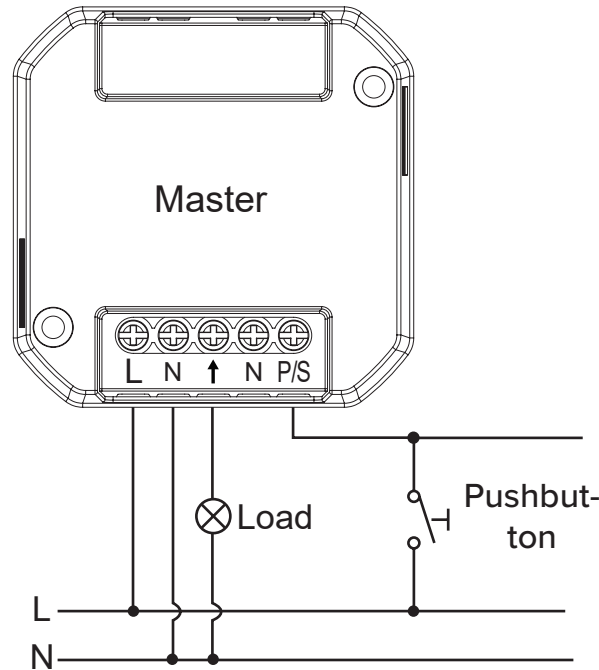
With pushbutton
